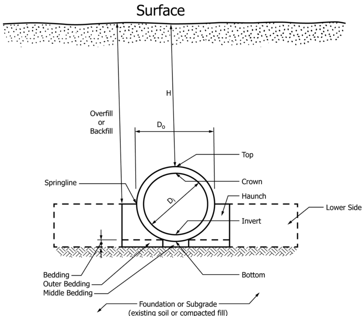
FIG. 1 Pipe/Installation Terminology
