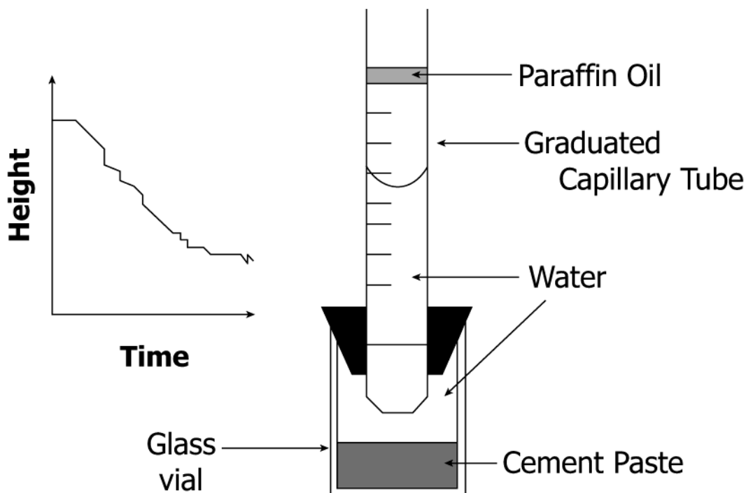
FIG. 1 Illustration of One Experimental Setup for Monitoring Chemical Shrinkage of Hydrating Cement Paste Using Procedure A.
