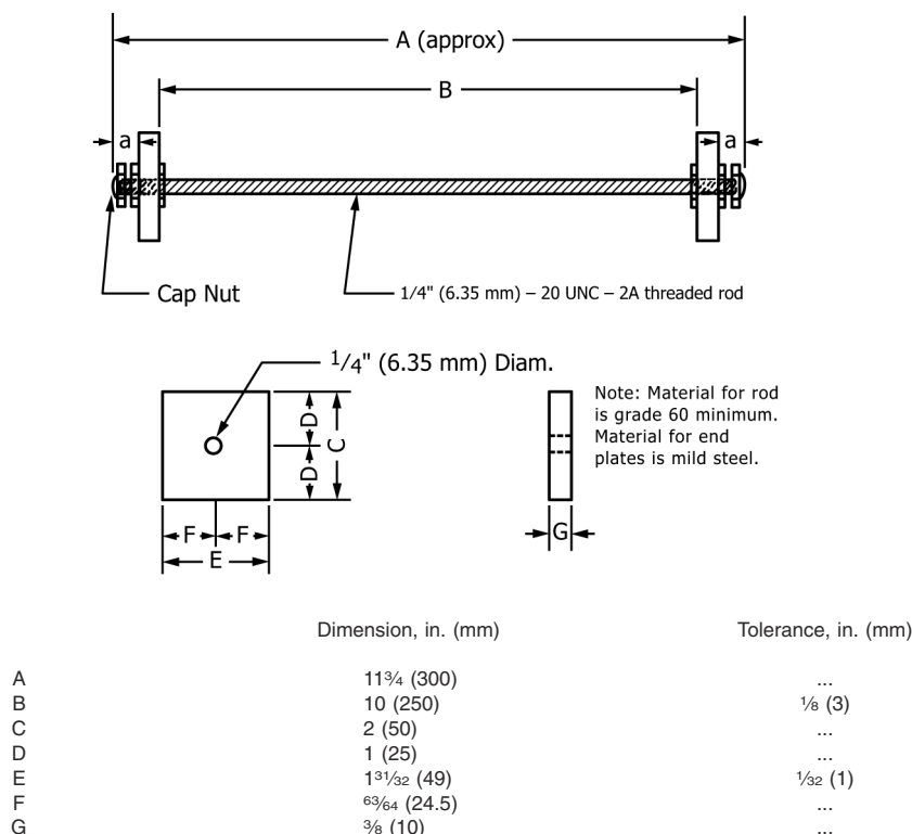
FIG. 1 Restraining Cage
