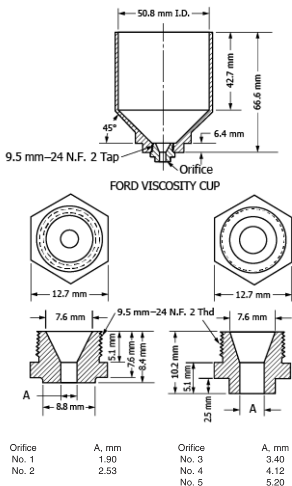
FIG. 1 Ford Viscosity Cup and Orifices
