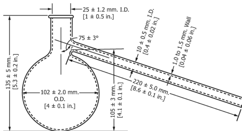
FIG. 1 Distillation Flask
