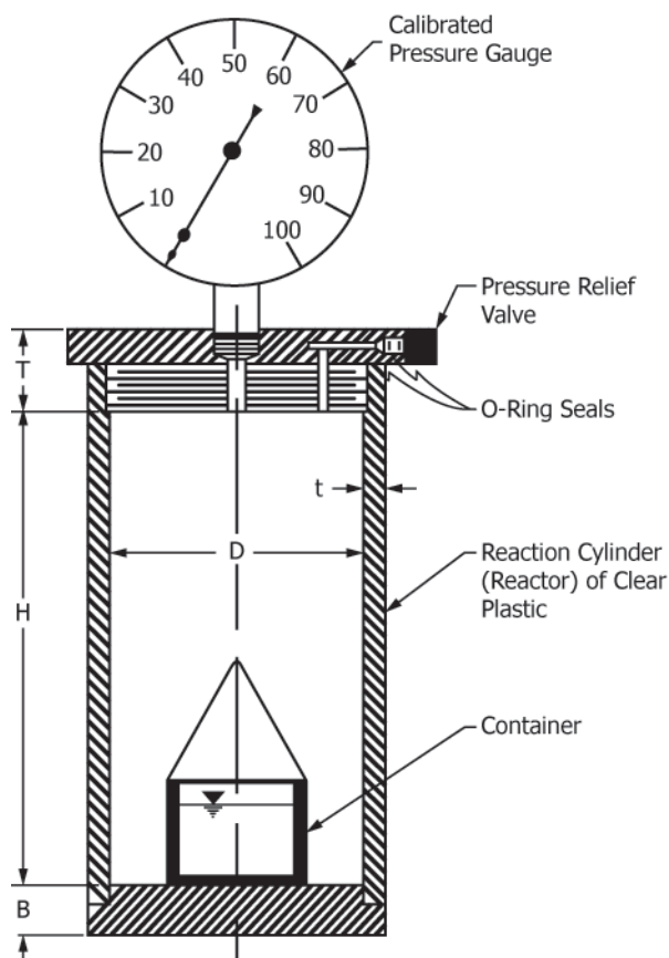
FIG. 1 Schematic Drawing of Rapid Carbonate Analyzer
