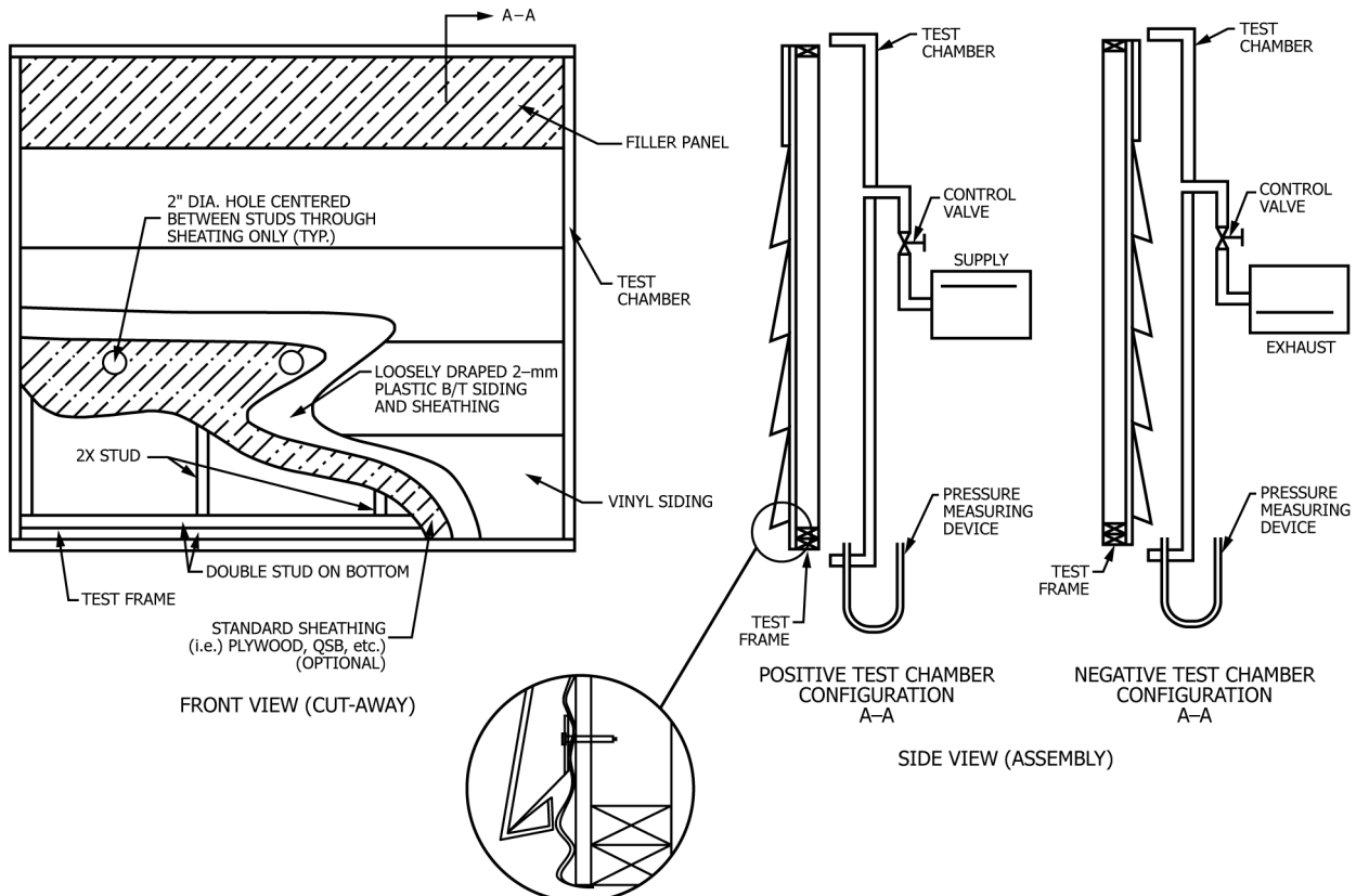
FIG. 1 Test Chamber
