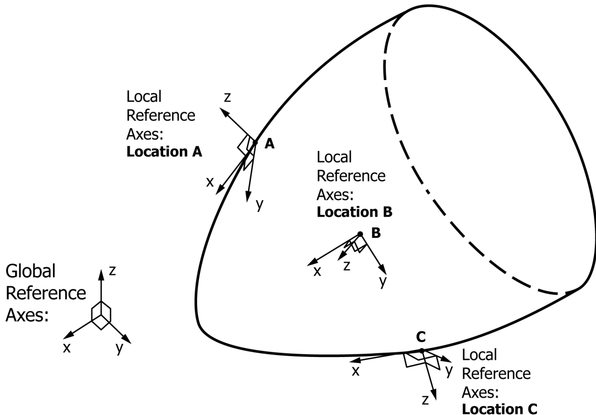
FIG. 1 Illustration of Possible Global and Local Reference Coordinate Axes for a Three-Dimensional Part
