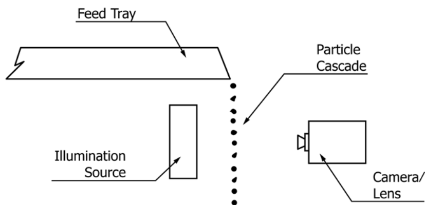
FIG. 1 Typical Apparatus
