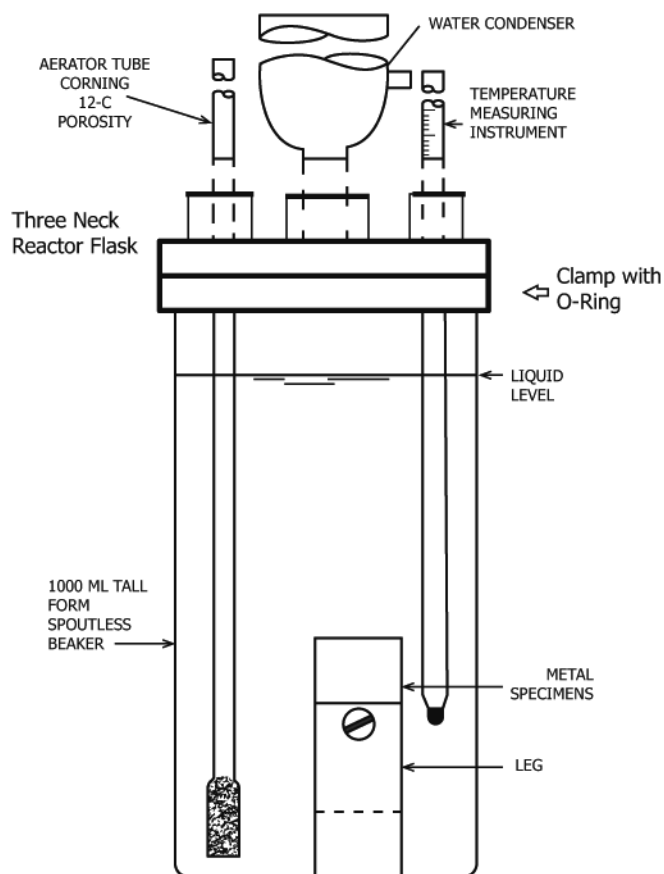
FIG. 1 Metal Specimens and Equipment for the 336 h Corrosion Test
