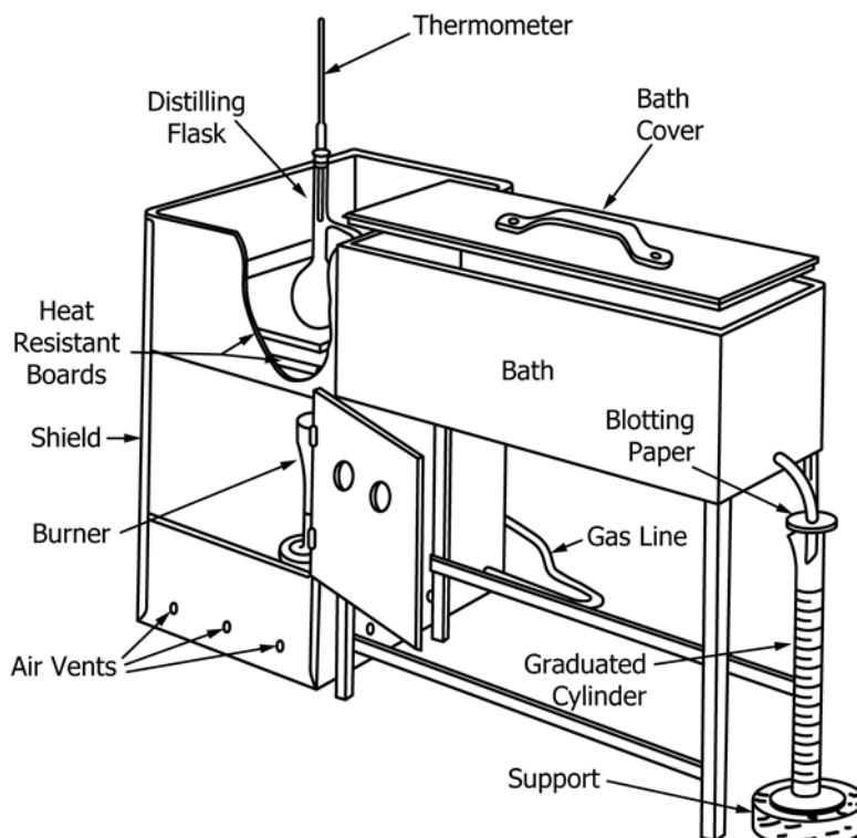
FIG. 1 Apparatus Assembly Using Gas Burner
