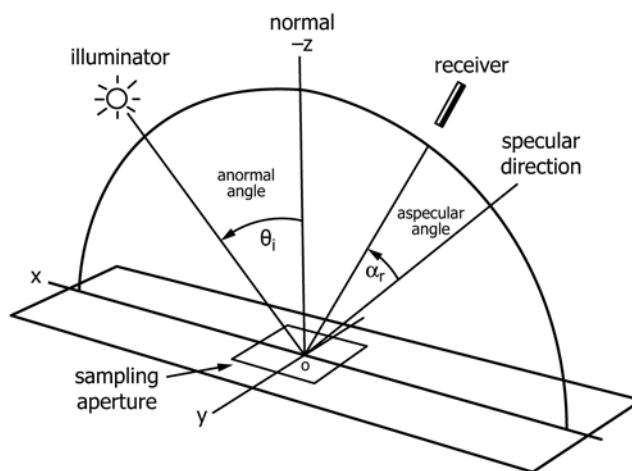
FIG. 1 Uniplanar Configuration
