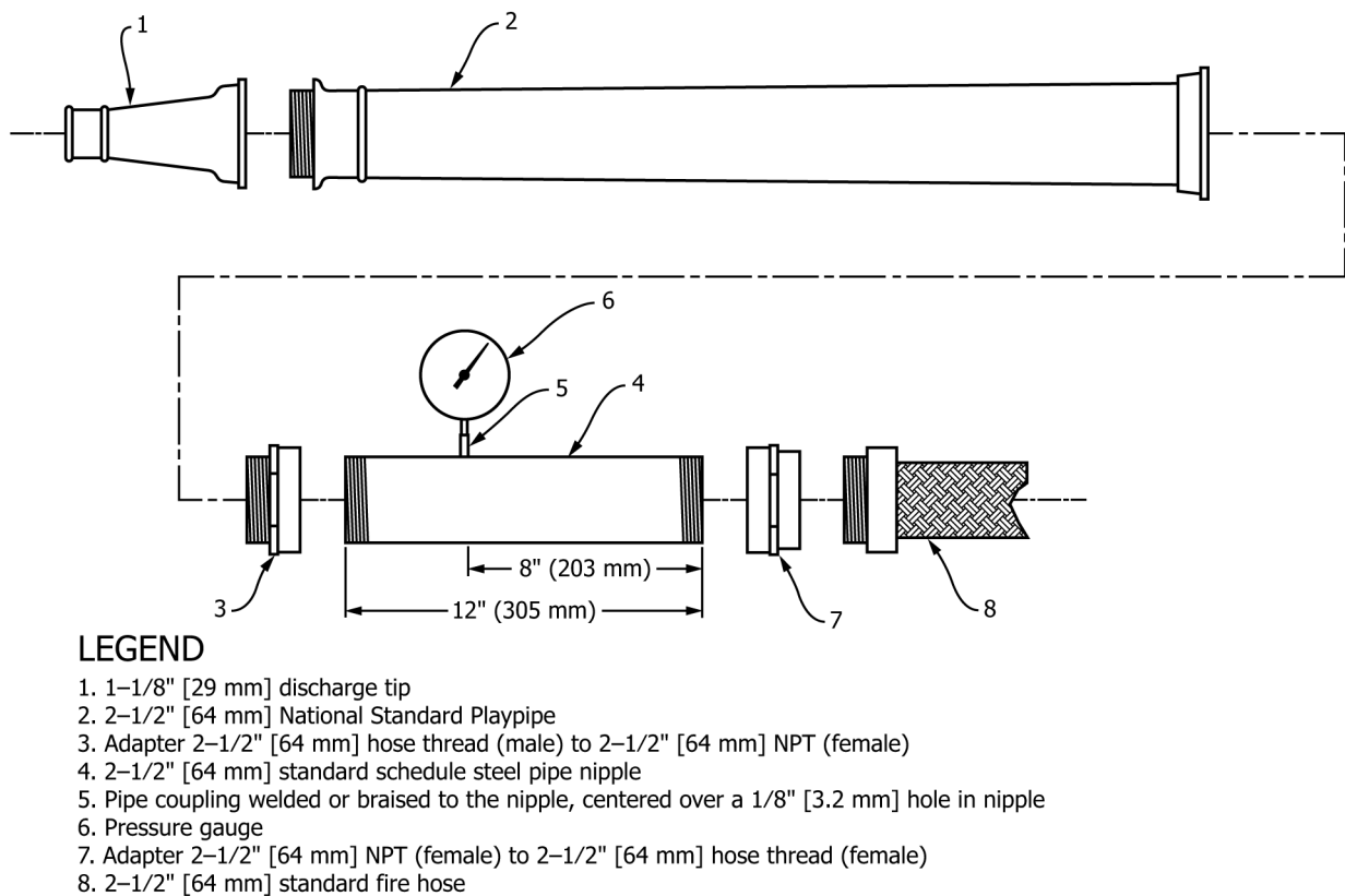
FIG. 1 Hose Stream Apparatus
