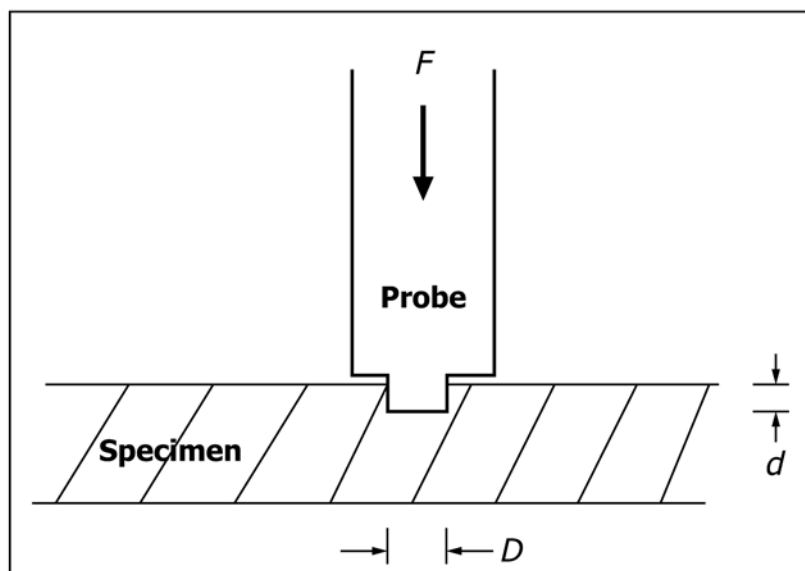
FIG. 1 Penetration Probe
