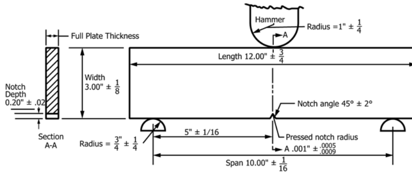
FIG. 1 Drop-Weight Tear Test Specimens and Support Dimensions and Tolerances (for Specimens \frac{1}{8} in. to \frac{3}{4} in. in Thickness)
