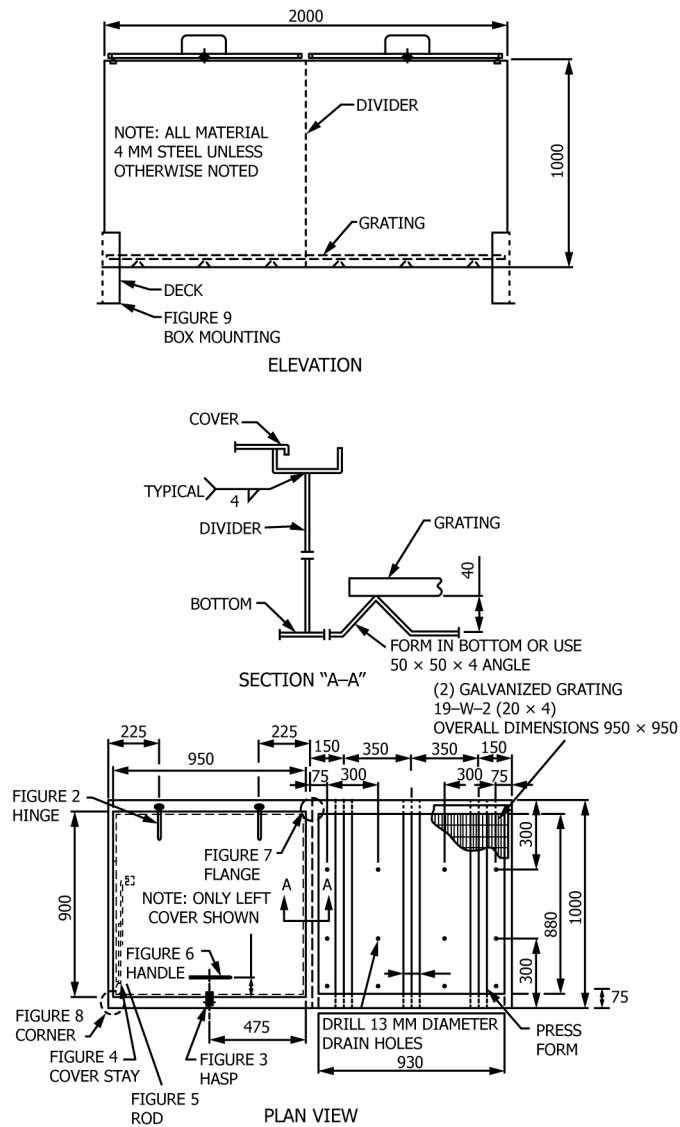
FIG. 1 Steel Deck Gear Stowage Box
