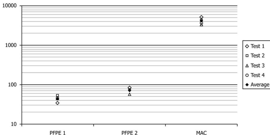
FIG. 1 Relative lifetimes of three typical space lubricants at 23°C in vacuum on 52100 steel
