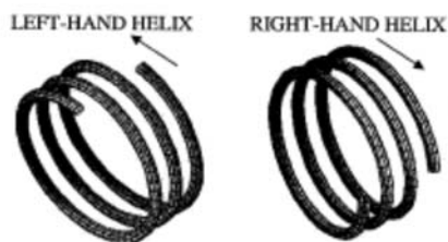
FIG. 1 Standard Definitions for Cast, Helix, and Camber of Spooled Wire
