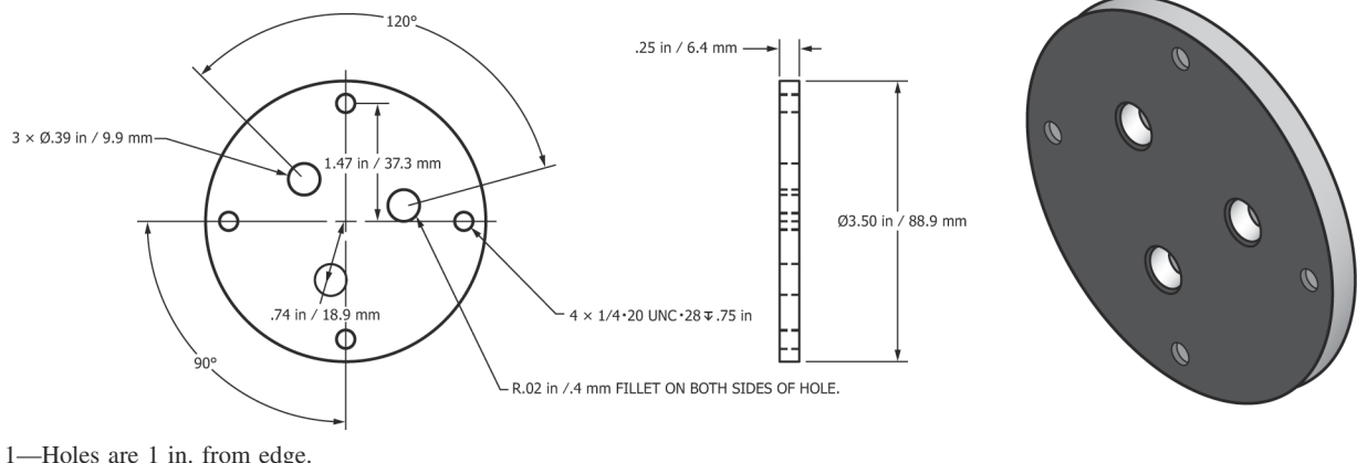
FIG. 1 Example of a Specimen Support Assembly (Two Needed)
