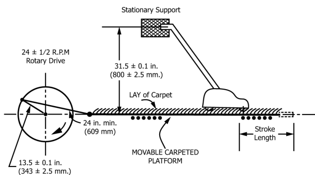
FIG. 1 Test Fixture
